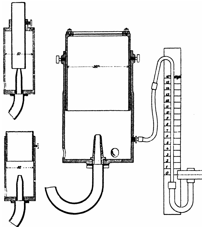
Figure A.4.1 Prüsmann's test equipment
