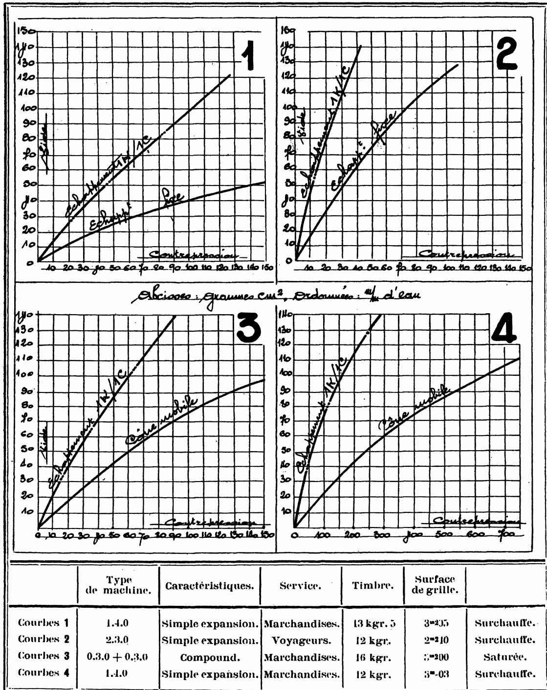
Figure A.24.7 Vacuum-Counterpressure graphs for different locomotives
