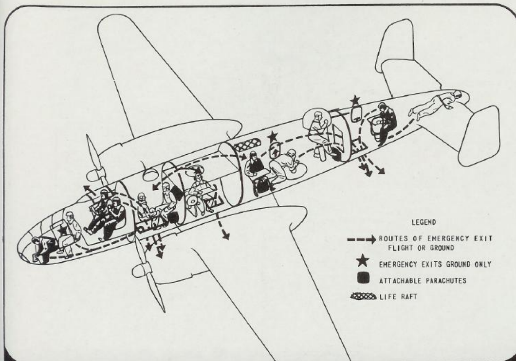
Figure 48 - Emergency Exits and Movement of Flight Personnel
